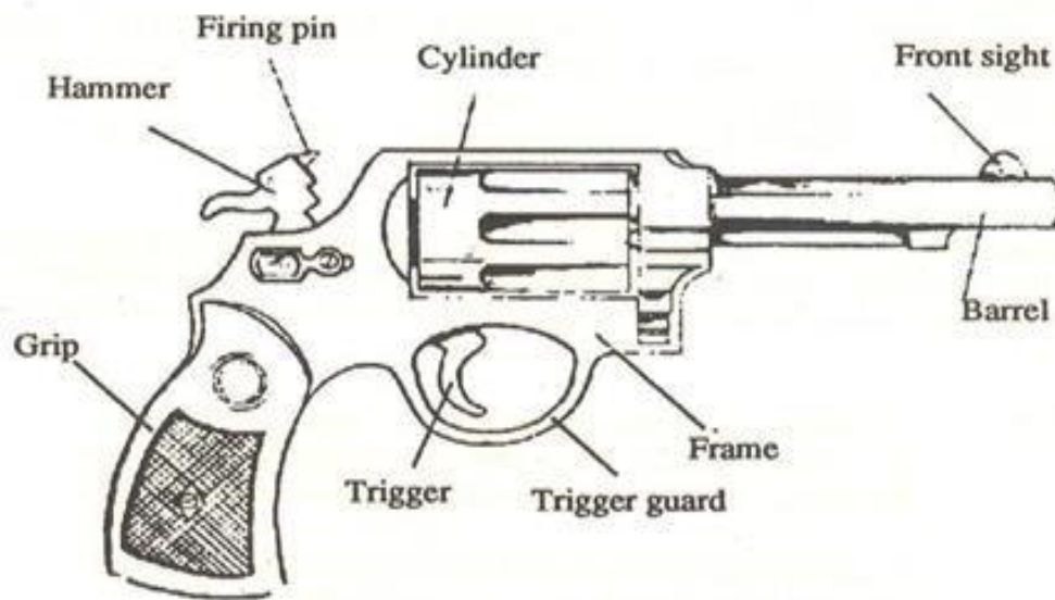
FIG. THE PARTS OF A REVOLVER
