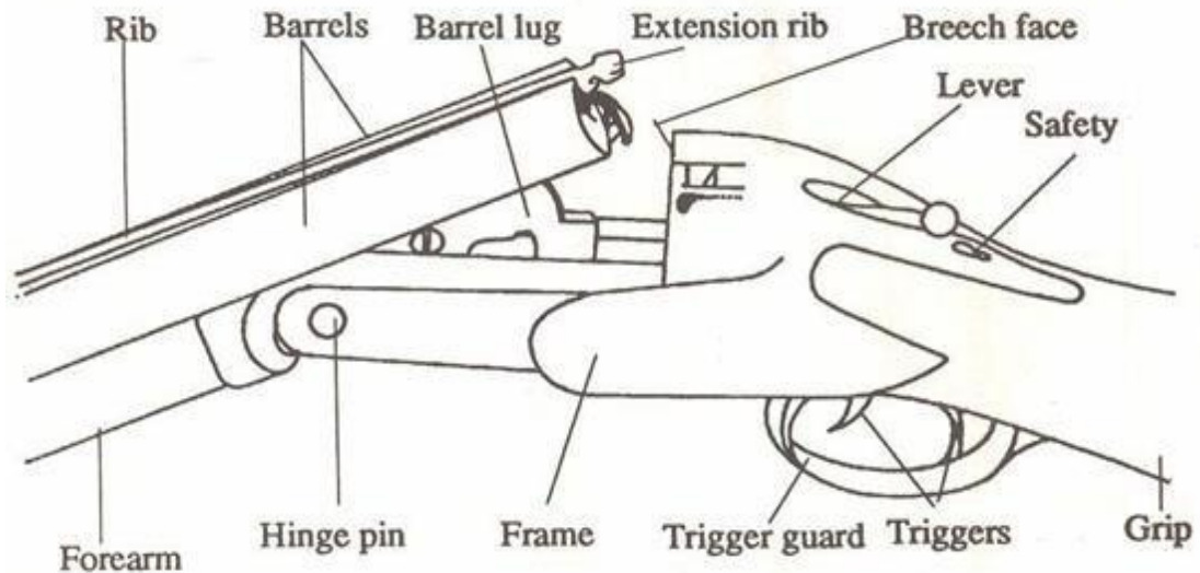
SCHEMATIC DIAGRAM OF DOUBLE BREECH LOADING GUN
